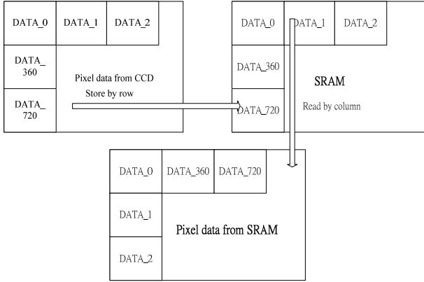
Figure 3. Transposition of pixel data from rows to columns
