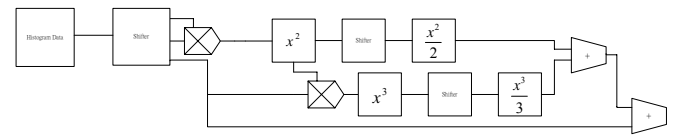
Figure 5. The architecture of log calculation unit
