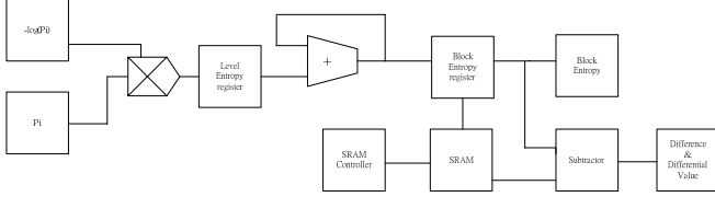
Figure 6. The architecture of the entropy calculation unit
