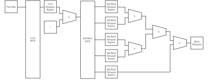
Figure 4. The architecture of the Gray level histogram calculation unit
