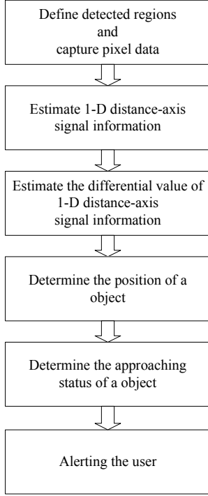
Figure 1. Algorithmic process of approaching vehicle detection
